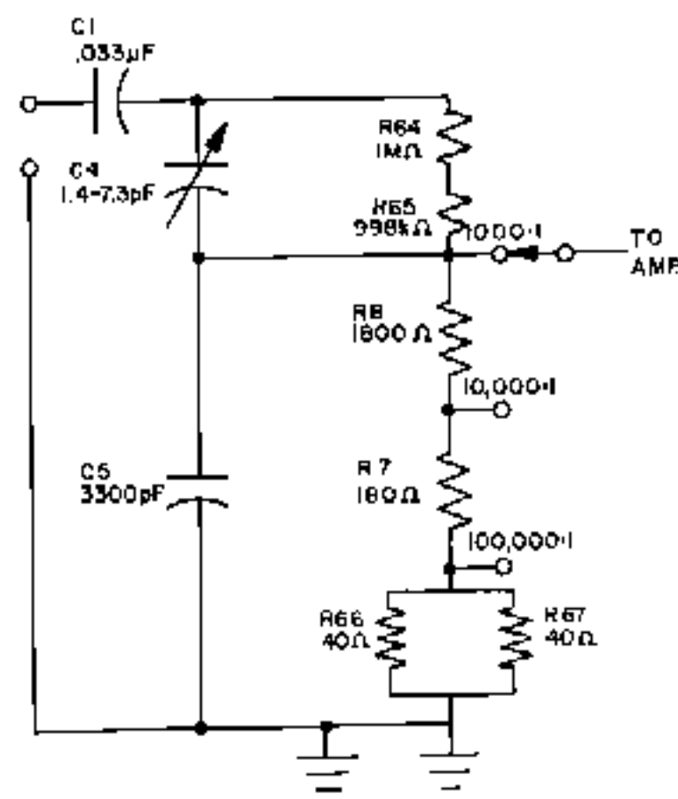
Fig. 4. Attenuator, Simplified Schematic
