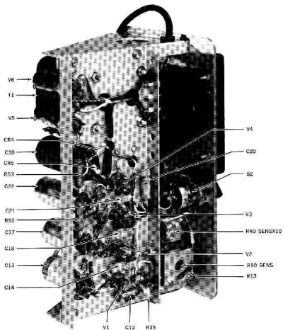
Fig. 7. Ballantine Model 300H-U7 Interior View, Left Side
