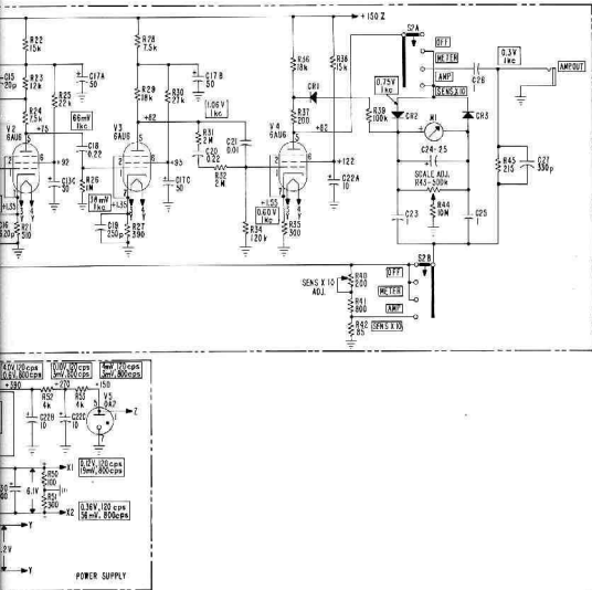
FIG. 9. SCHEMATIC DIAGRAM, ISSUE No. MD-3451A MODEL 300H-U7 SENSITIVE ELECTRONIC VOLTMETER
