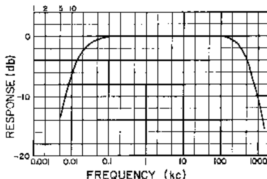
Fig. 3. Typical Frequency Response of SENS X10 Function
