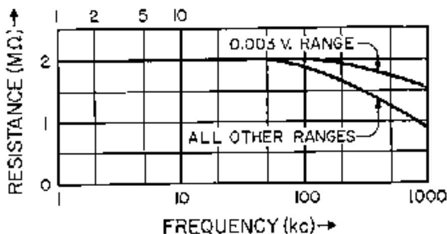
Fig. 2. Typical Input Resistance vs. Frequency
