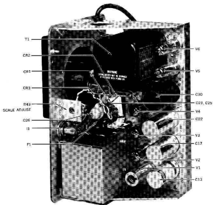
Fig. 8. Ballantine Model 300H-U7 Interior View, Right Side
