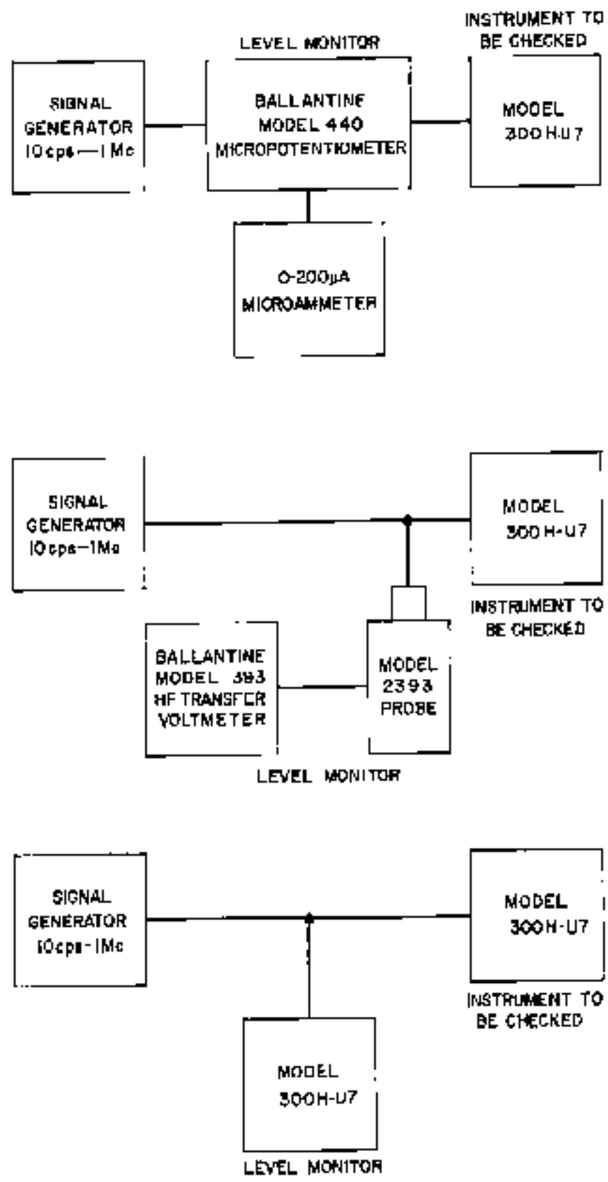
Fig. 6. Frequency Response Check
